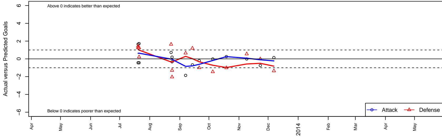
Kent United Black B00 Dots are actual minus expected GF (blue circles) and GA (red triangles). Blue line is smoothed change in attack strength. Red is smoothed change in defense strength.
